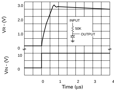
Transient Response ( I_R=150\mu A )
