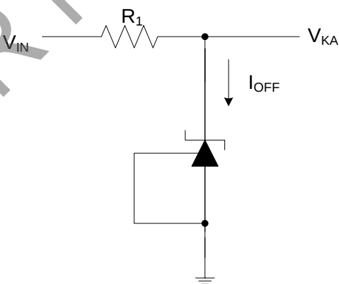
Test Circuit 6 for I_{OFF}
