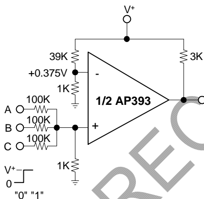
AND Gate
