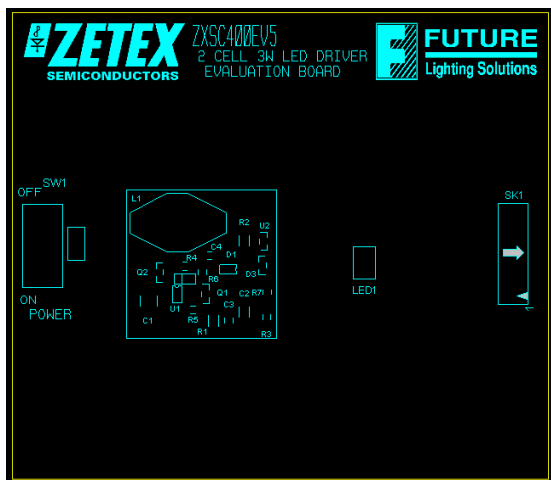
Top Silk
