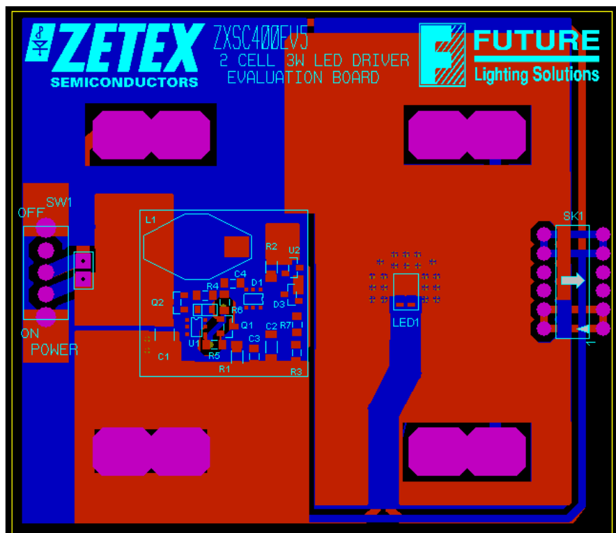
Figure 4. Evaluation PCB
