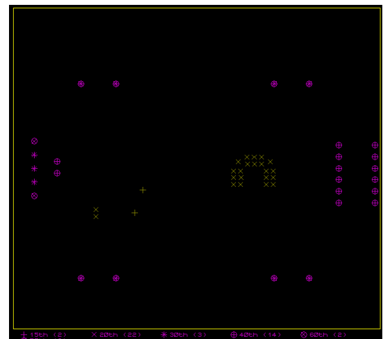
Drill File
