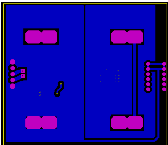
Bottom Copper
