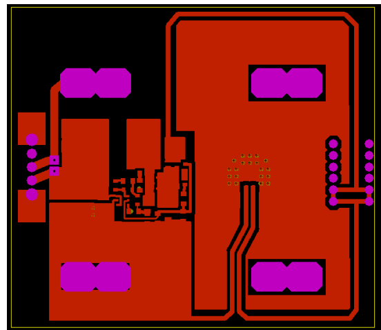
Top Copper
