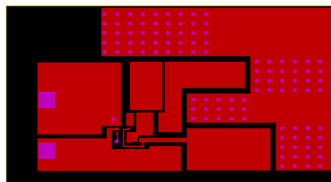
Top Copper
