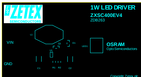
Top Silk
