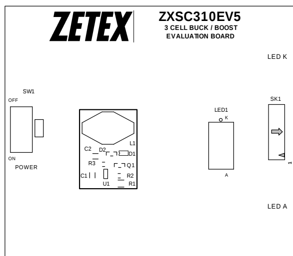
Top Silk
