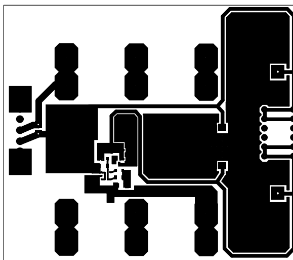
Top Copper
