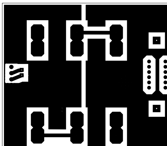
Bottom Copper
