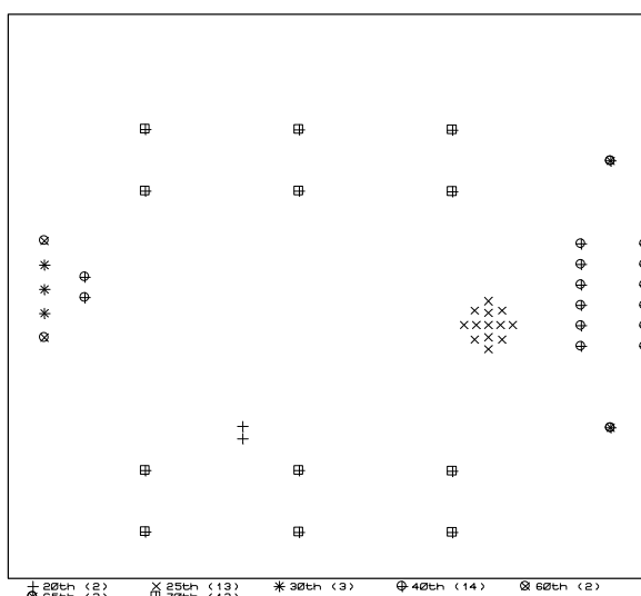
Drill File
