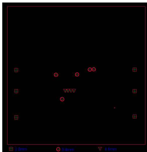
Drill File
