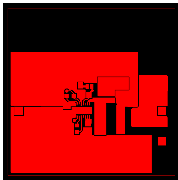
Top Copper
