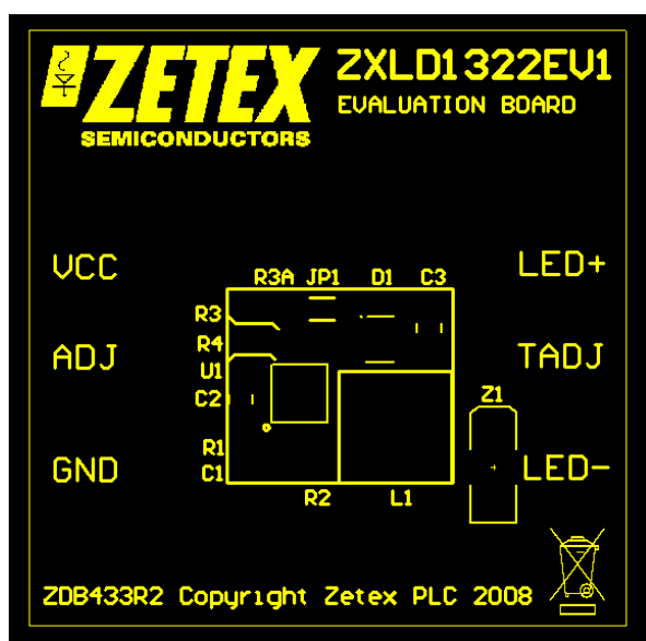
Top Silk
