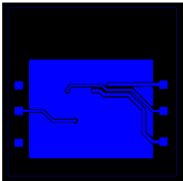
Bottom Copper
