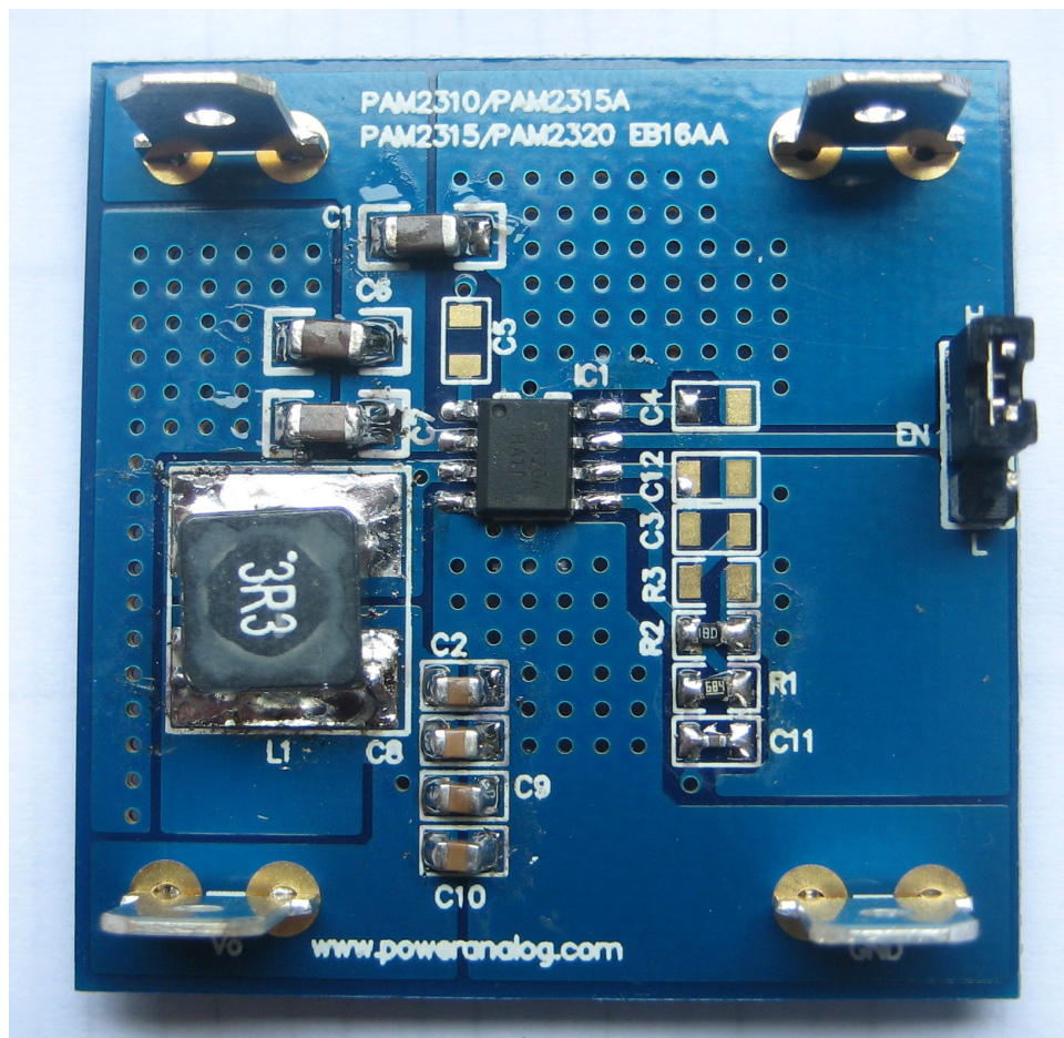
Top View
