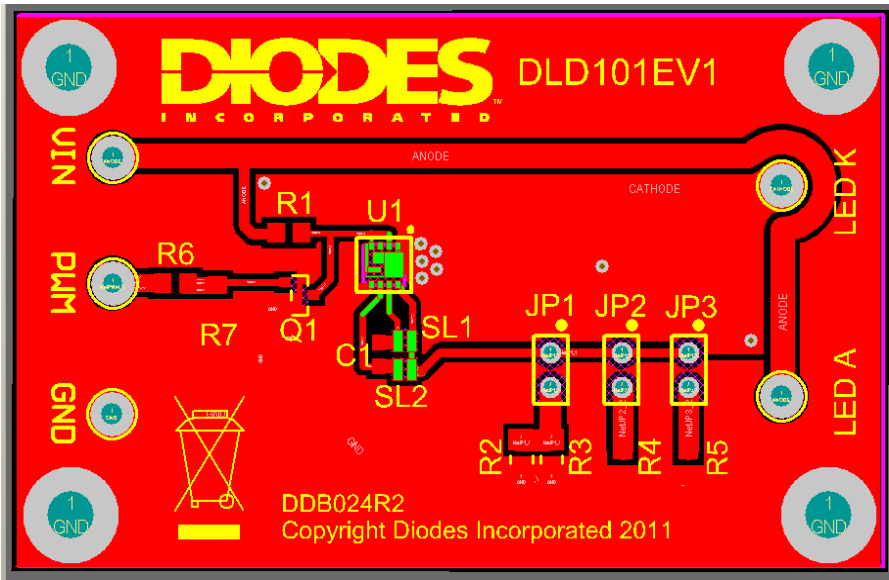
Figure 7. PCB layout
