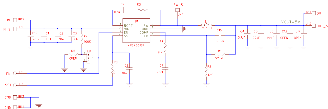
Figure 3. AP64351SP-EVM Schematic
