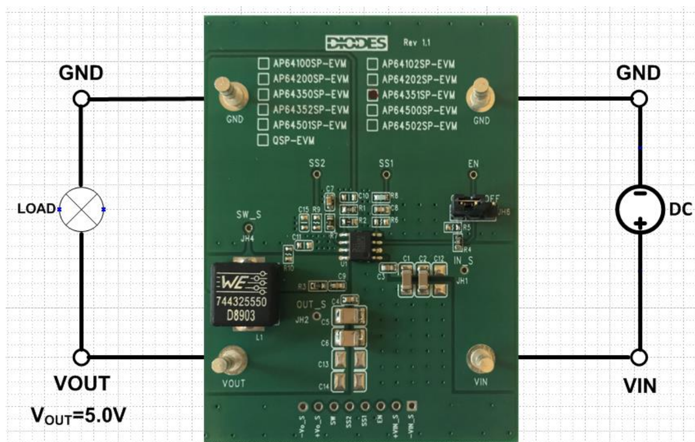
Figure 2. AP64351SP-EVM
