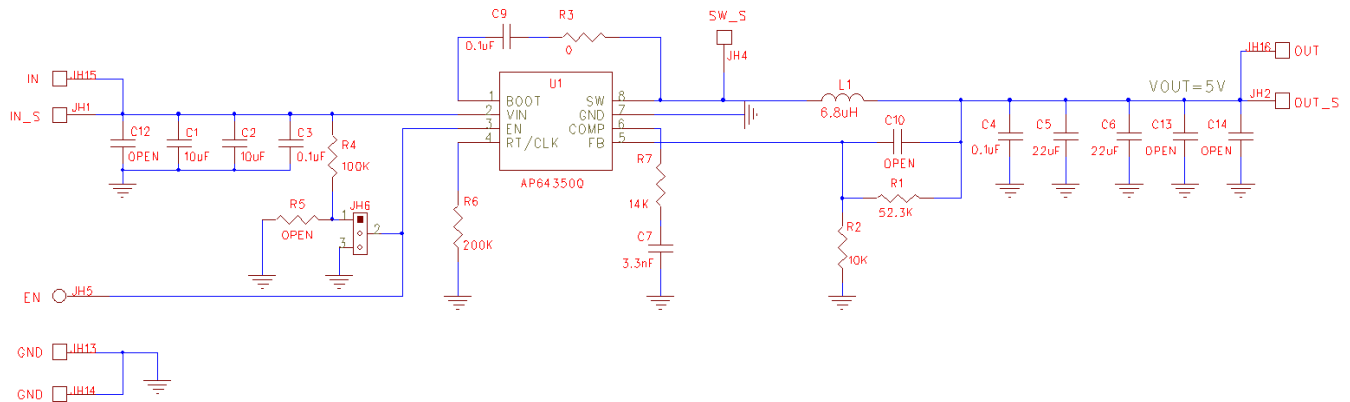
Figure 3. AP64350QSP-EVB Schematic
