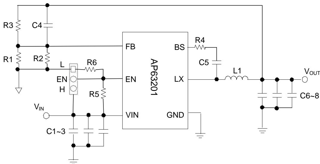
Figure 3. AP63201WU-EVM Schematic
