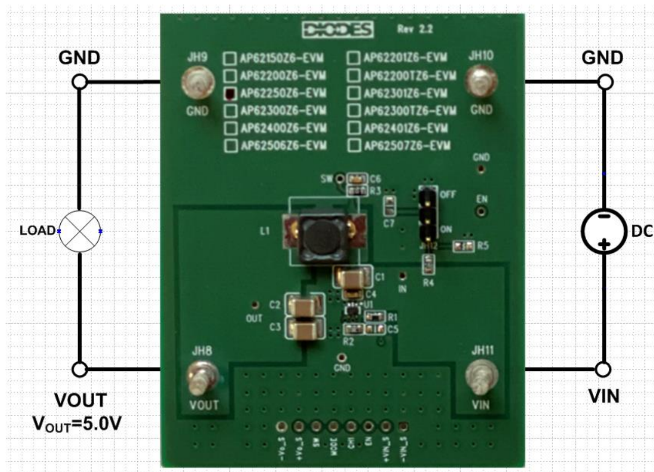
Figure 2. AP62250Z6-EVM
