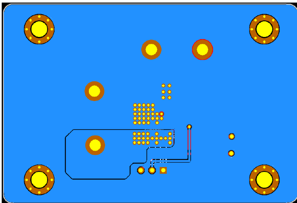
Figure 4. AP61302Z6 - EVM - Bottom Layer
