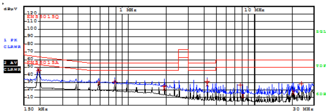
Figure 6: CISPR 15 Conducted Emissions Plot, 150 kHz to 30 MHz, VIN = 40 V, IOU T = 3A, 6LEDs
