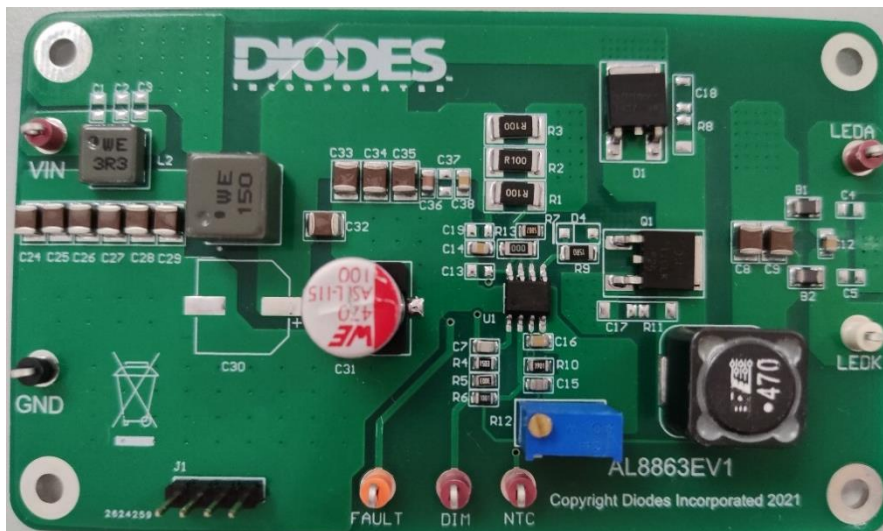
Figure 1: Top View
