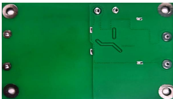
Figure 2: Bottom View
