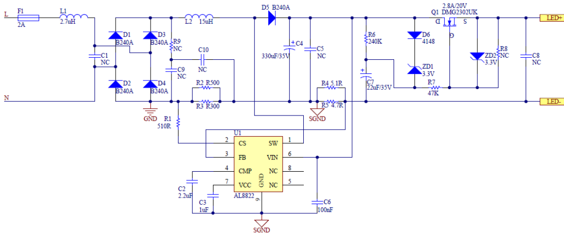
Figure 5: Schematic Circuit
