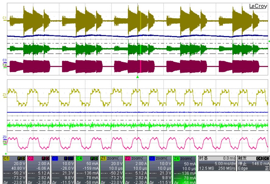
Waveform #3 – Minimum Dimming with dimmer GUNG => I_4=0\text{mA}
