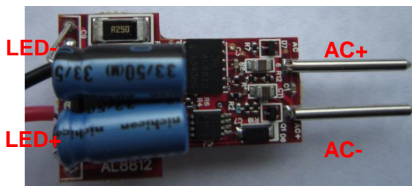
Figure 1: Top View
