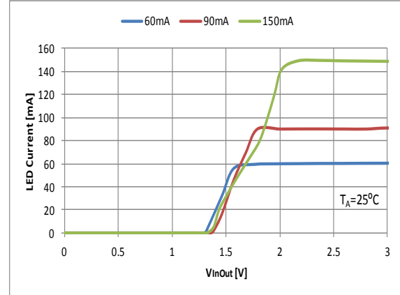
Figure 8. Startup Minimum Operating Voltage
