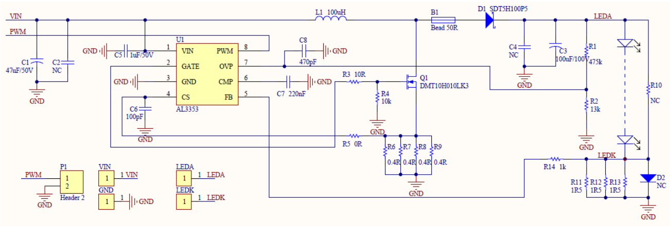
Figure 5: Schematic Circuit
