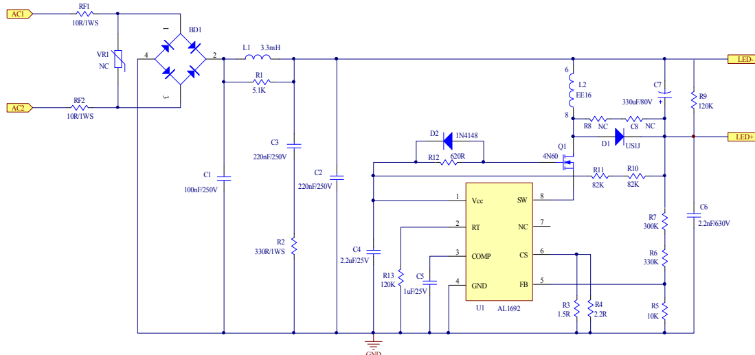
Figure 5: Schematic Circuit
