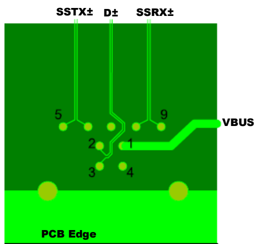
Figure 13: Example of routing on Standard-B receptacle connector
