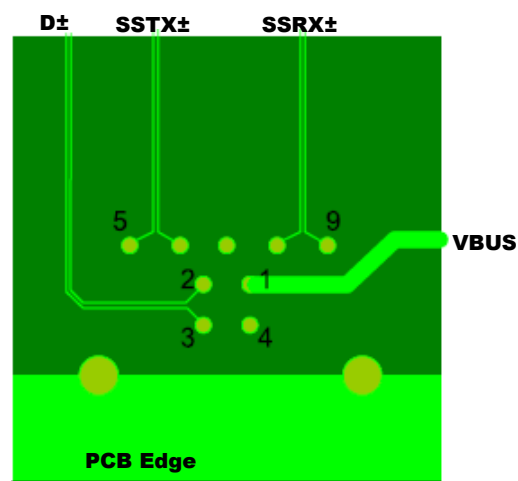
Figure 13: Example of routing on Standard-B receptacle connector
