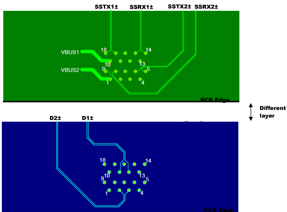
Figure 14: Example of routing on Standard-A double-stack connector
