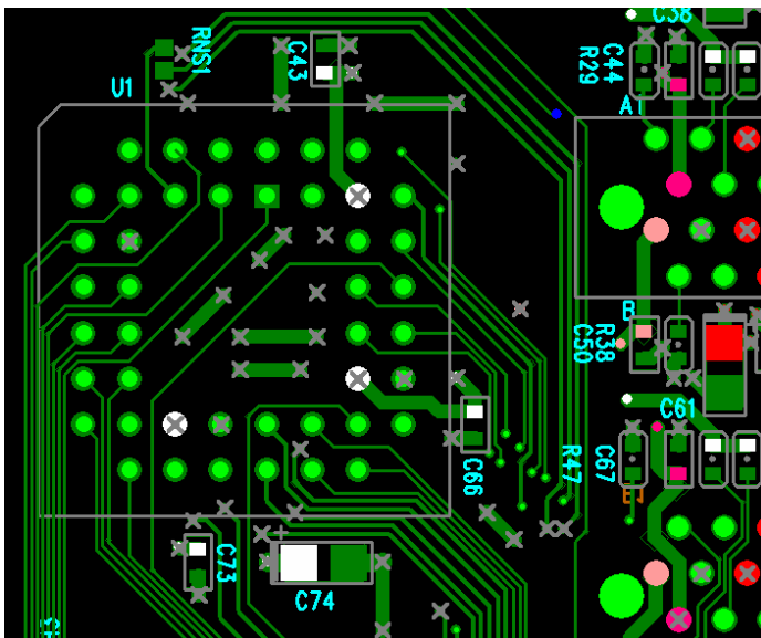
Figure 2: Detail of top layer near external arbiter clock and req/gnt enter at lower left
