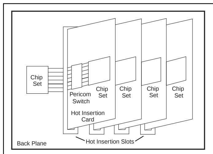
Figure 4. Hot-Swap Application using Pericom Switches
